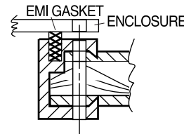
Figure 7 Through Hole Style 3033
